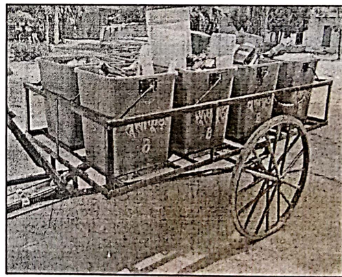
Tricycle with 8 Detachable Bins
